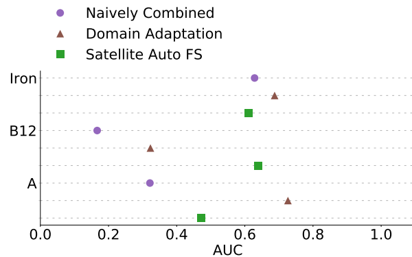
Figure 6: Comparing AUC of a logistic regression model trained by naively combining training data from all regions, a multi-layer perceptron with domain adaptation, and a region-specific logistic regression model, all in CP.
