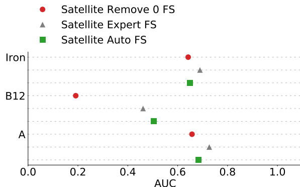
Figure 4: Comparison feature selection methods, including removing any bands without data, human expert feature selection, and our K-medoids method, all in region WCO.
